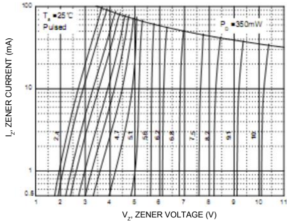
Temperature Coefficients
