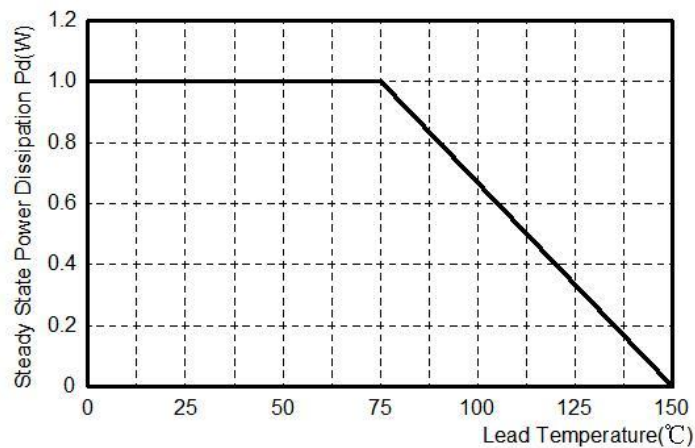
FIG5: Steady State Power Dissipation
