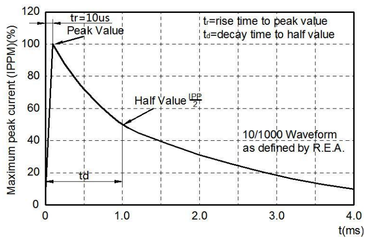
FIG3: Pulse Waveform
